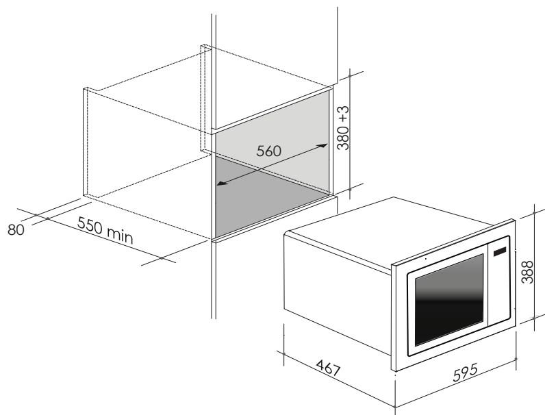
WALLMOUNT INSTALLATION
