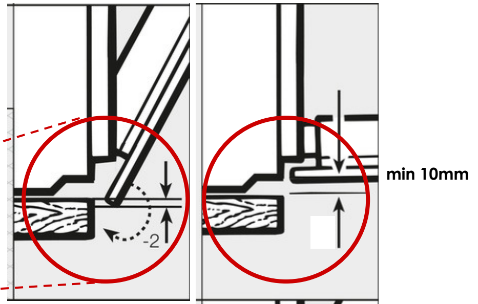
Door opening at 45°
